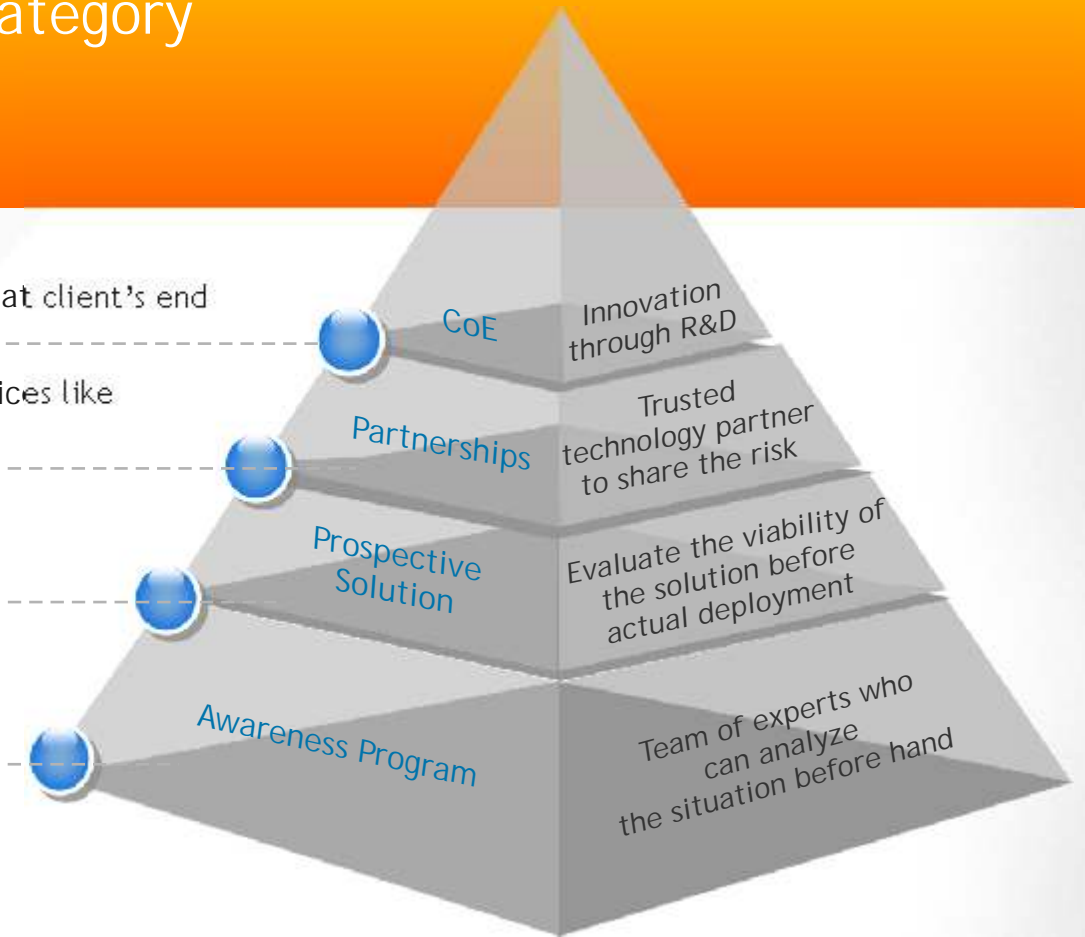
ENGAGEMENT MODEL
